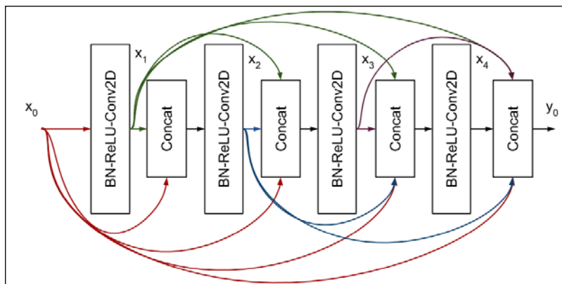
Figure 2.4.1: A 4-layer Dense block in DenseNet.
