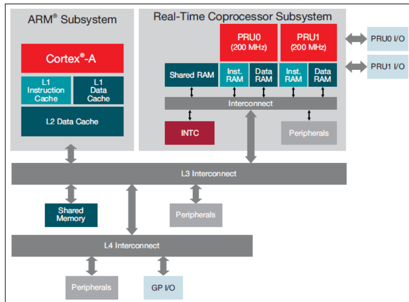
PRUs exist as parallel but distinct processors on the board
