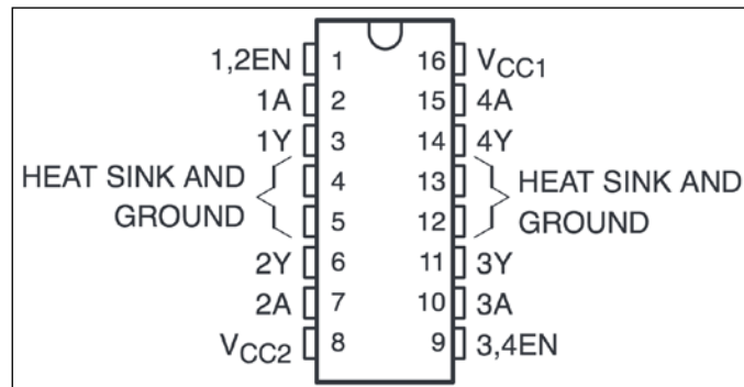
Pin outs on H-bridge
