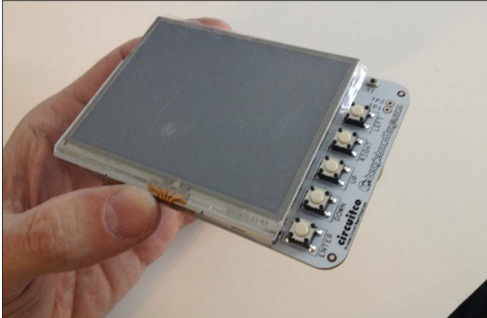
CircuitCo LCD3 cape
