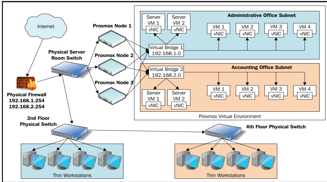
Visualizing the same campus with a Proxmox VE virtualized network infrastructure
