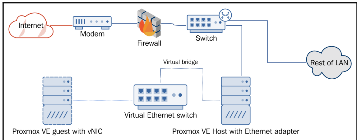
Visualizing bridged configuration
