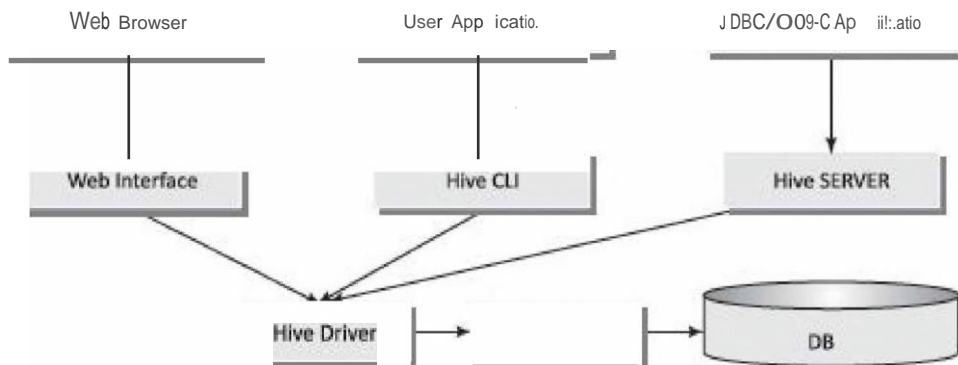
Figure4.10 Hive architecture
