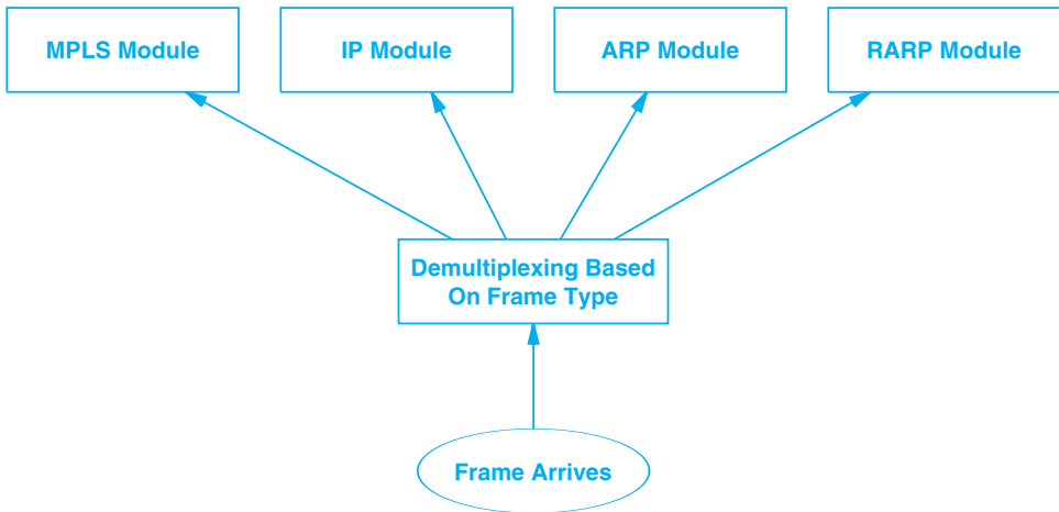
Figure 16.5 Frame demultiplexing in an LSR that handles both MPLS and conventional IP forwarding.
