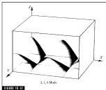
Three-dimensional representation of the sound pressure distribution in a rectangular room for the tangential mode (2,1,0), from Acoustic Instruments, Inc.
