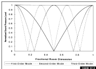
Normalized energy distribution of the first three modes in a room.
