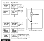
Block diagram of ETP's impulse response measurement methodology. (Courtesy of Deep Fluid, AboutSoft.)
