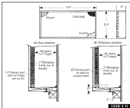
FIGURE 9-41 Plan for a practical module absorber utilizing the wall as the bottom of the module. (Left) Bass absorber. (Right) Wideband absorber.
