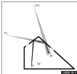
Second-order reflection of sound S from surfaces (D) and (E) to receiver (R) using cone tracing. S1 and S2 are virtual sources.
