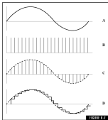
FIGURE 6-7 [A] the analog signal, [B] digitizing pulses, [C] the digitized analog signal, resulting from the modulation of [A] with [B], Application of a sample-and-hold circuit to [C] which completes the quantization process reducing the analog samples to discrete values suitable for storage in memory.
