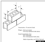
Staggered stud concrete block construction.
