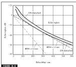
FIGURE 18-8 Acceptable echo levels for speech under reverberant conditions. (Reverberation Time 1.1 seconds). (After Wallace, Barron, and Isenhardt.)
