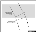
Rays of sound traveling from a denser medium having a higher sound speed into a less dense medium having a lower sound speed. The wavefront AB is not parallel to wavefront AC because the direction of the wave is changed due to refraction.
