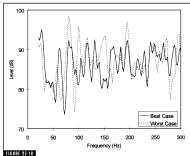
FIGURE 27-18 Comparison between the model response for two listening and loudspeaker arrangements of a full-dipole configuration.
