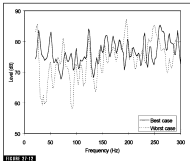
FIGURE 27-12 Long-term spectrum. The standard deviations are 1.85 and 4.28 dB for the best solution and the worst case, respectively.
