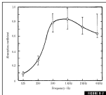
The average absorption characteristics of 8 oz/sq ft glass fiber material of 1-in 2 thickness. The vertical lines show the spread of the data.
