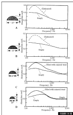
Measured absorption of polycylindrical diffusers of various chord and height dimensions. In C and D, graphs are shown for both empty polycs and for polycs filled with mineral wool. In A and B only empty polyc data are available; the broken lines are estimated absorptions when filled with mineral wool. (After Mathewsky 10 )
