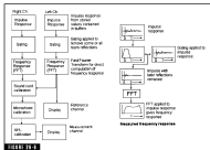
Block diagram of EAS 3D frequency response measurement methodology. (Courtesy of Doug Reed, AcoustiSoft.)
