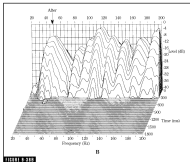
Low-frequency modal structure of the sound field of the same small room after the introduction of the forced Helmholtz resonator structure.
