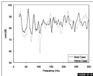
Comparison of the model response for two listener and loudspeaker arrangements of a stereo pair with two woofers per loudspeaker.
