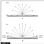
FIGURE 12-4 Comparison of refraction of sound from source in (A) cool air near the ground and warmer air above, (B) warm air near the ground and cooler air above. In (B) note that sound shadow areas result from the upward refraction.
