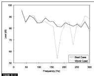
FIGURE 27-12 Comparison of the speaker-boundary interference response for two listener and loudspeaker arrangements of five optimally matching loudspeakers.
