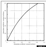
FIGURE 9-4 An approximate relationship between the absorption coefficients at normal incidence and those with random incidence.
