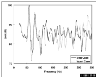
Comparison of the model response for the two listener and loudspeaker arrangements of the equivalent matching loudspeakers.
