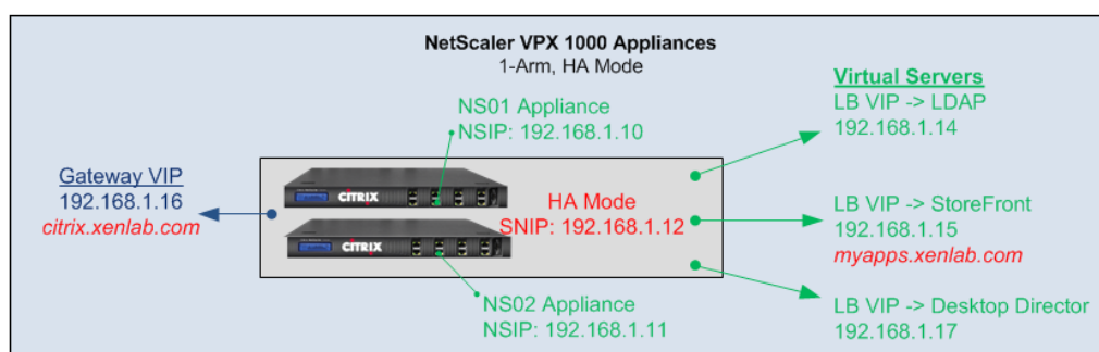
NetScaler connections planning diagram
