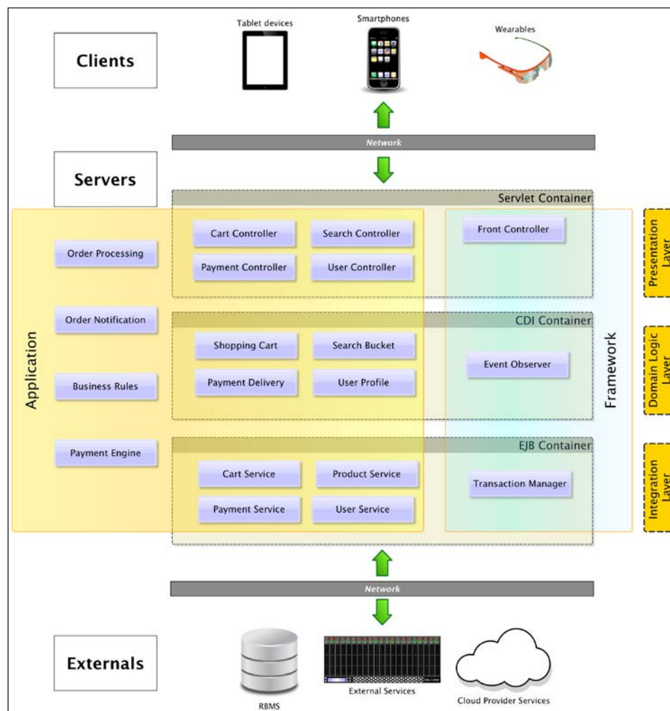
The standard Java EE web architecture
