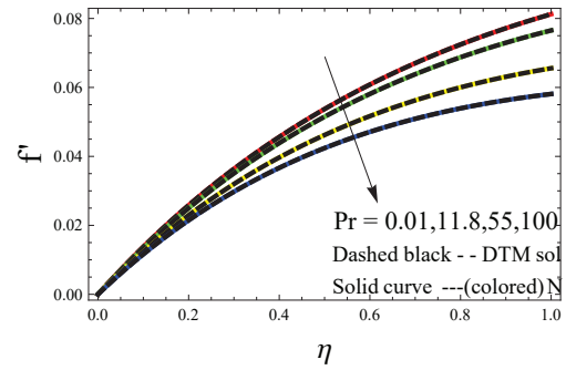
FIGURE 5. Velocity profile of the fluids for different values of P_r
