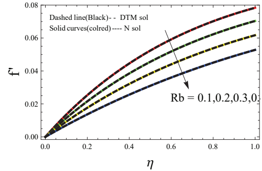
FIGURE 3. Velocity profile of the fluids for different values of the parameter R_b
